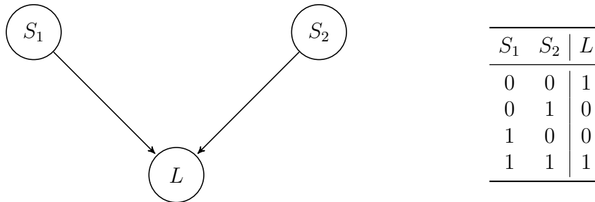
Figure 1: Graphical representation of the circuit example.
